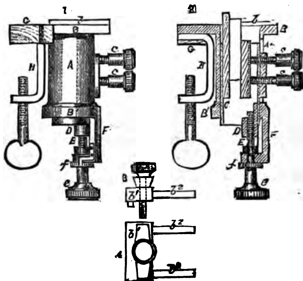
Halles's Microtome.
